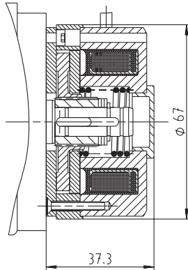
Motor type 13.120/13.710
